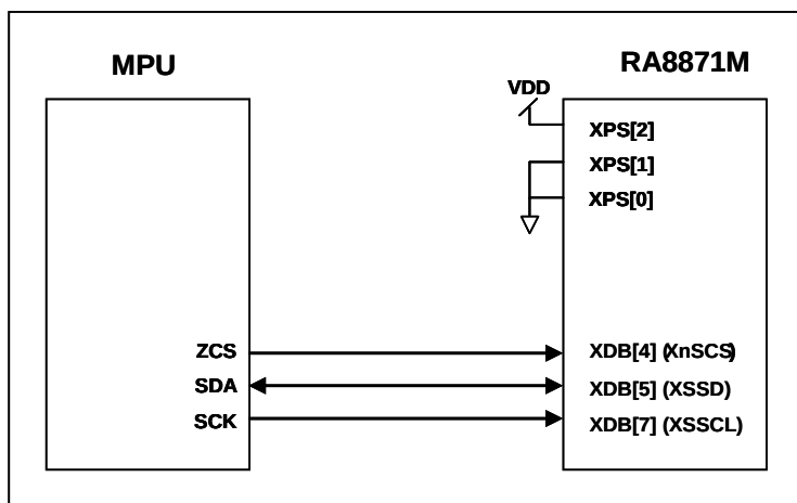
圖 7-7 : The MPU Interface Diagram of 3-Wire SPI
